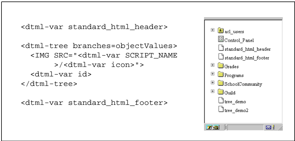
Figure 13. Use of the branches tag to display all sub-objects in a folder.
