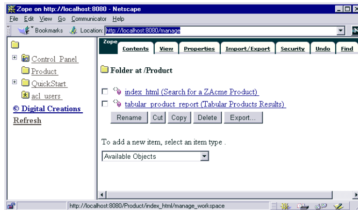
Figure 11. Contents view of the Products folder after adding a tabular search interface.
