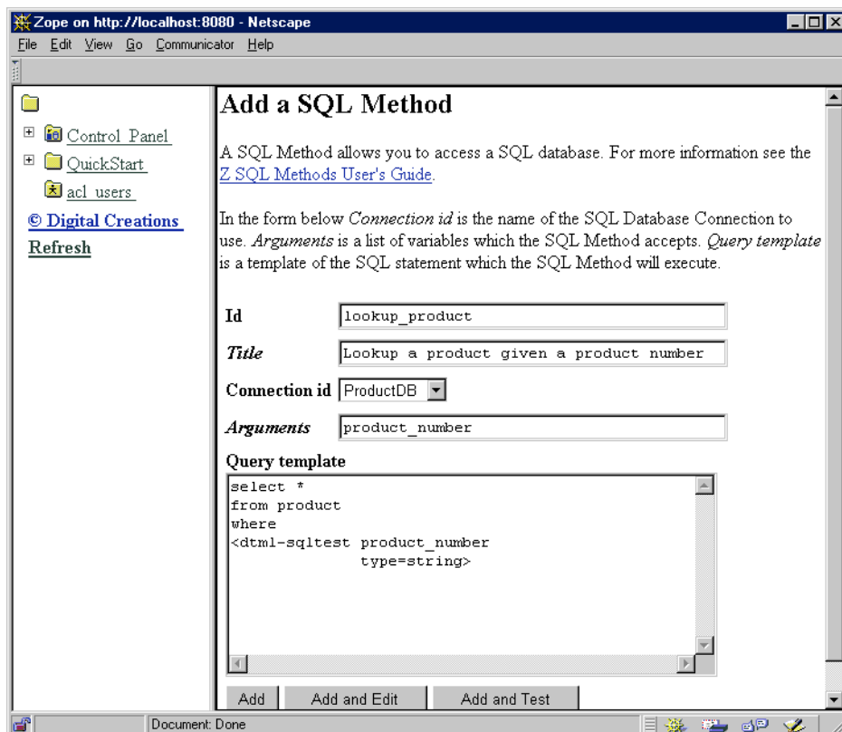
Figure 7. Add SQL method for Product Query
